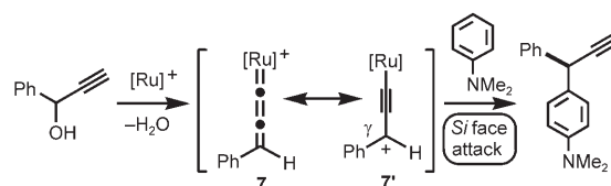
Scheme 4. Attack of the aromatic compound on the Si face at the Cy atom of the allenylidene complex.
